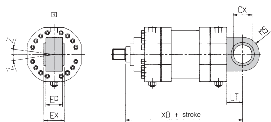
Swivel attachment with eye: S (ISO MP5)
