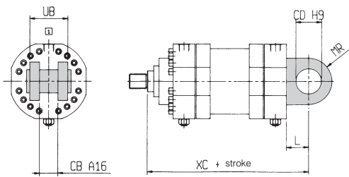
Female clevis attachment: C (ISO MP1)
