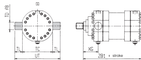
Front-body trunnion: G (ISO MT1)
