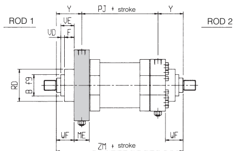
Front flange execution for double-rod: N
