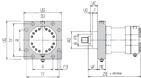
Front flange attachment: N (ISO MF5)
