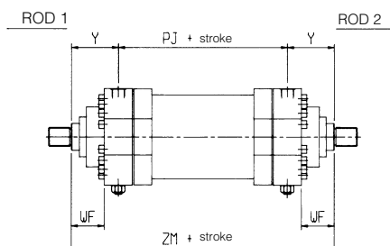
Basic execution for double-rod: X (double-rod execution can be supplied for G-L-N attachments)
