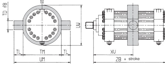
Mid-body trunnion: L (ISO MT4) tie-rod fastening
