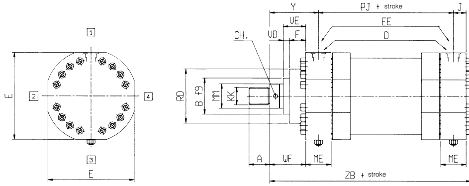
Basic configuration: X - cushioning adjustment on side 3
