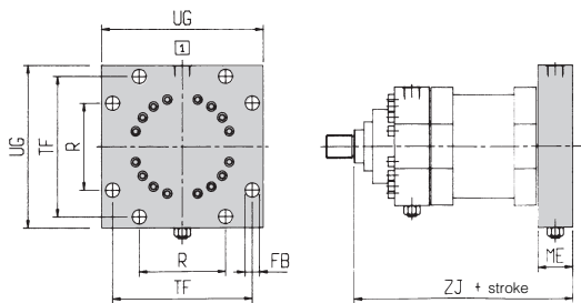
Rear flange attachment: P (ISO MF6)
