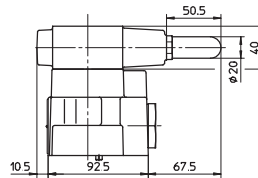
AGIS-10: Mass = 3,8 Kg AGISR-10: Mass = 4 Kg AGIU-10: Mass = 3,8 Kg
