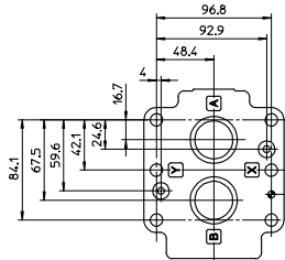
AGIR-32: Mass = 9,4 Kg AGIRR-32: Mass = 9,6 Kg
