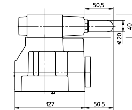
AGIS-20: Mass = 6 Kg AGISR-20: Mass = 6,2 Kg AGIU-20: Mass = 6 Kg
