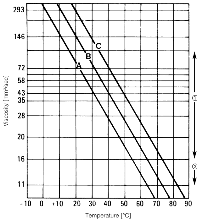
Figure 5 Viscosity Vs. Temperature graph
